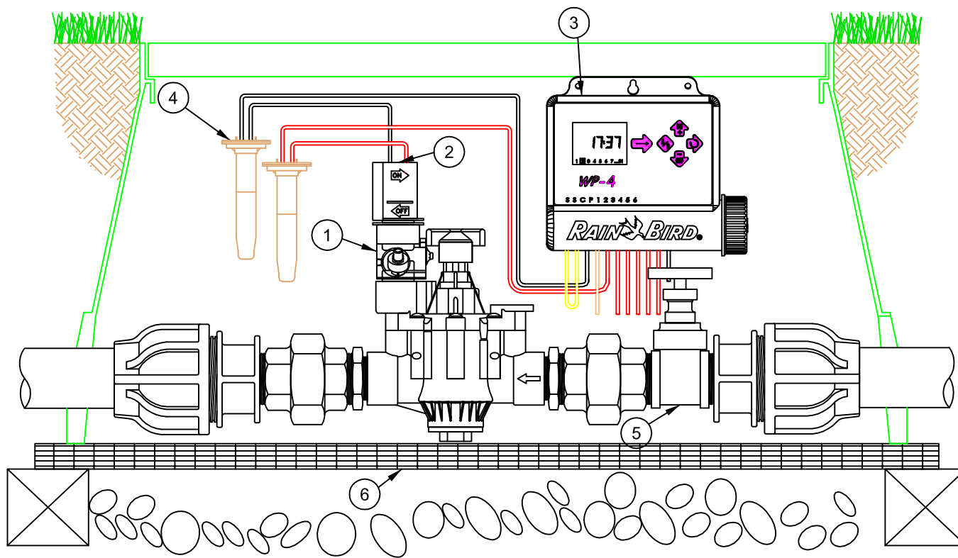
PGA VALVE + PRS-DIAL / WP-2/4/6/8
